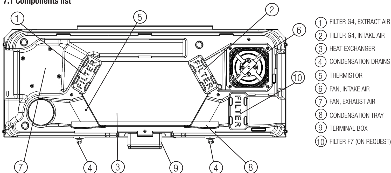
Fig. 7.a Internal components
