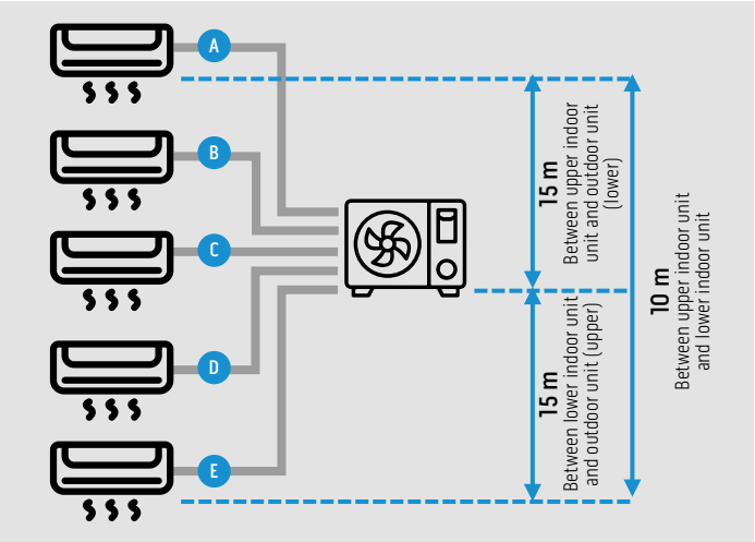
Maximum distance single pipes Indoor unit to Outdoor unit
