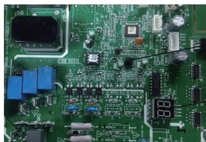
Correct
