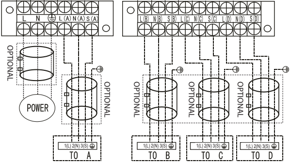
CASSETTE
