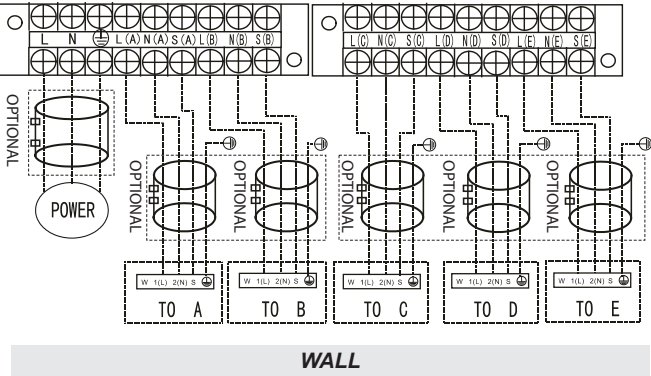
WALL
