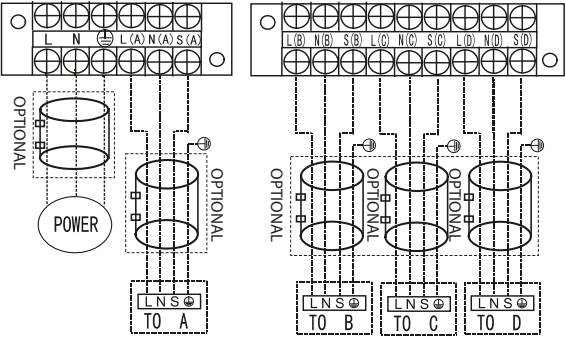
DUCT
