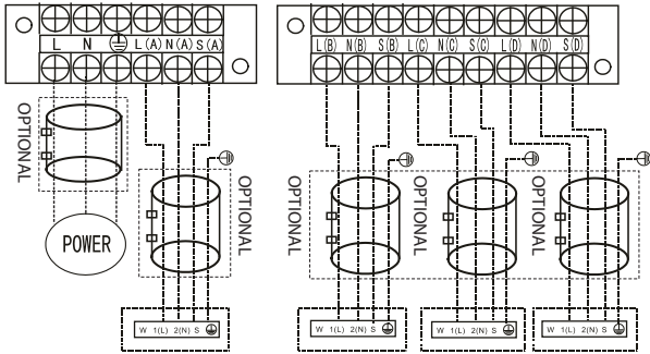
WALL
