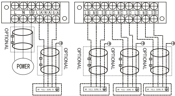
WALL
