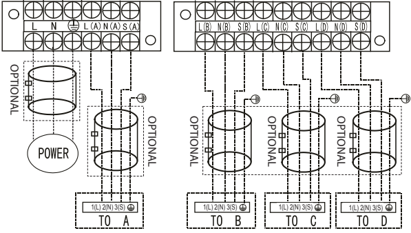
CASSETTE
